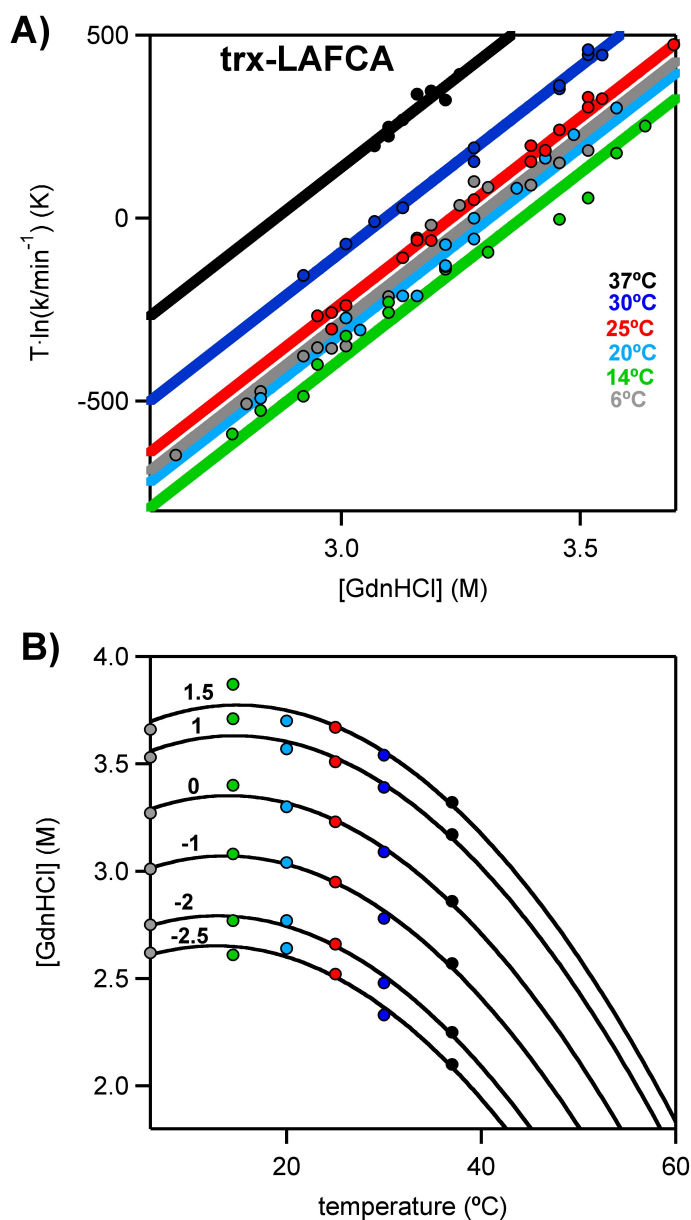
Fig. S5. Determination of the temperature-dependent unfolding rate constant for LAFCA thioredoxin at zero guanidine concentration. Guanidine-induced denaturation experiments were performed at several temperatures and guanidine concentrations. (A) Linear extrapolation to zero guanidine concentration to obtain the values of rate constants at lower temperatures. (B) Constant- \ln k_U extrapolation to obtain the values of the rate constants at higher temperatures. The color of the data points refers to the temperature, as shown in panel A. The lines are the best fits of second-order polynomials. The numbers alongside the lines stand for the \ln k_U values.
