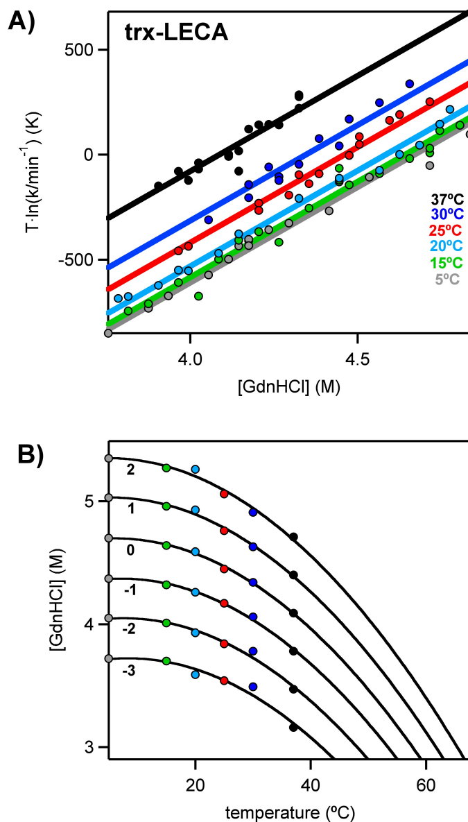
Fig. S6. Determination of the temperature-dependent unfolding rate constant for LECA thioredoxin at zero guanidine concentration. Guanidine-induced denaturation experiments were performed at several temperatures and guanidine concentrations. (A) Linear extrapolation to zero guanidine concentration to obtain the values of rate constants at lower temperatures. (B) Constant- \ln k_U extrapolation to obtain the values of the rate constants at the higher temperatures. The color of the data points refers to the temperature, as shown in panel A. The lines are the best fits of second-order polynomials. The numbers alongside the lines stand for the \ln k_U values.
