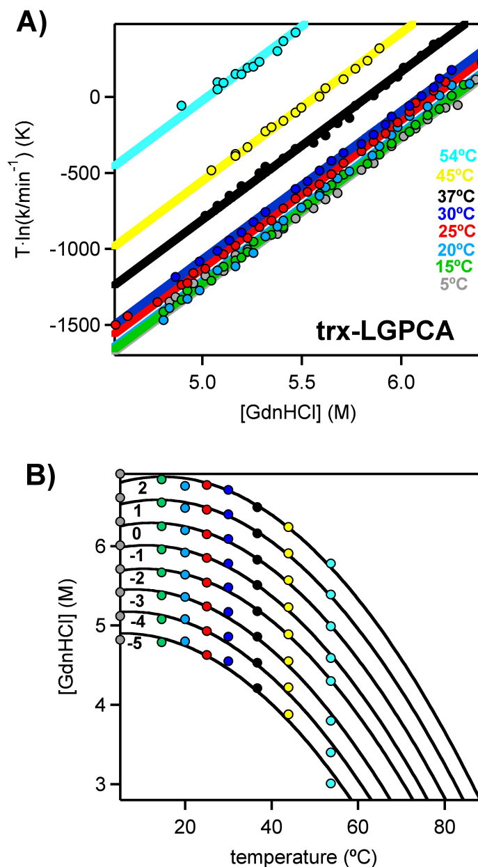
Fig. S7. Determination of the temperature-dependent unfolding rate constant for LGPCA thioredoxin at zero guanidine concentration. Guanidine-induced denaturation experiments were performed at several temperatures and guanidine concentrations. (A) Linear extrapolation to zero guanidine concentration to obtain the values of rate constants at lower temperatures. (B) Constant- \ln k_U extrapolation to obtain the values of the rate constants at higher temperatures. The color of the data points refers to the temperature, as shown in panel A. The lines are the best fits of second-order polynomials. The numbers alongside the lines stand for the \ln k_U values.
