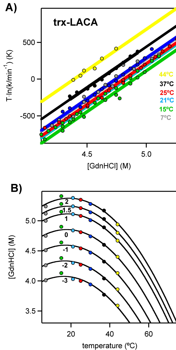
Fig. S9. Determination of the temperature-dependent unfolding rate constant for LACA thioredoxin at zero guanidine concentration. Guanidine-induced denaturation experiments were performed at several temperatures and guanidine concentrations. (A) Linear extrapolation to zero guanidine concentration to obtain the values of rate constants at lower temperatures. (B) Constant- \ln k_U extrapolation to obtain the values of the rate constants at the higher temperatures. The color of the data points refers to the temperature, as shown in panel A. The lines are the best fits of second-order polynomials. The numbers alongside the lines stand for the \ln k_U values.
