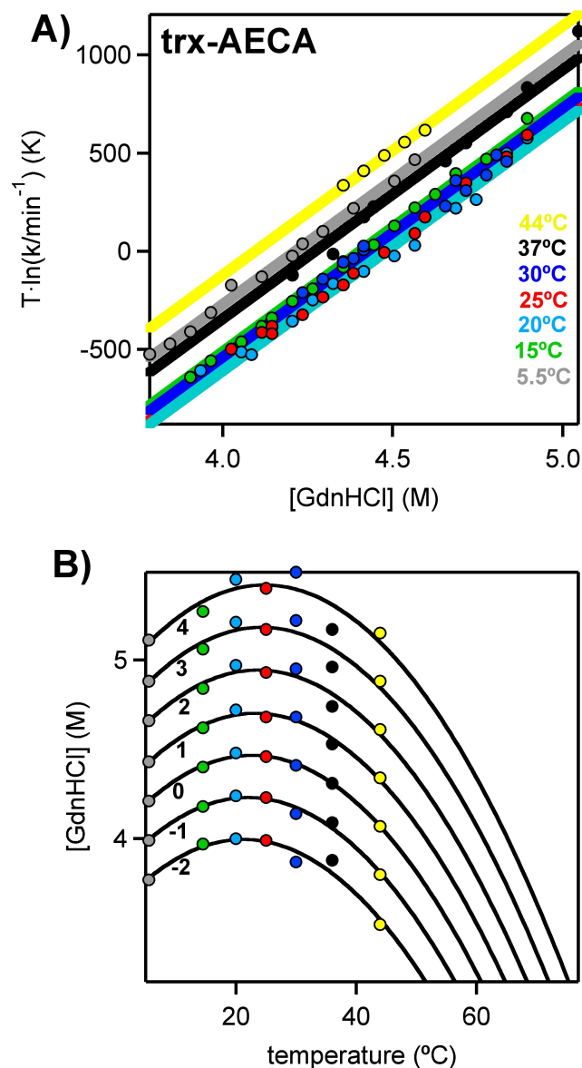
Fig. S10. Determination of the temperature-dependent unfolding rate constant for AECA thioredoxin at zero guanidine concentration. Guanidine-induced denaturation experiments were performed at several temperatures and guanidine concentrations. (A) Linear extrapolation to zero guanidine concentration to obtain the values of rate constants at lower temperatures. (B) Constant- \ln k_U extrapolation to obtain the values of the rate constants at the higher temperatures. The color of the data points refers to the temperature, as shown in panel A. The lines are the best fits of second-order polynomials. The numbers alongside the lines stand for the \ln k_U values.
