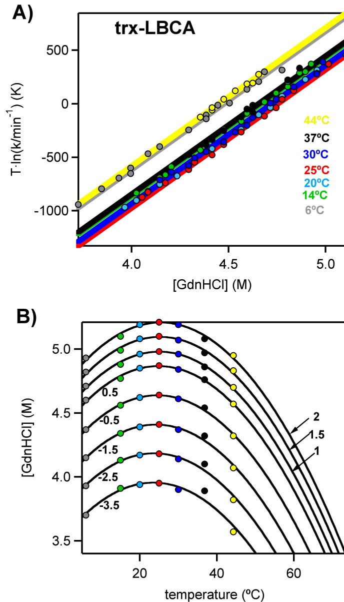
Fig. S11. Determination of the temperature-dependent unfolding rate constant for LBCA thioredoxin at zero guanidine concentration. Guanidine-induced denaturation experiments were performed at several temperatures and guanidine concentrations. (A) Linear extrapolation to zero guanidine concentration to obtain the values of rate constants at lower temperatures. (B) Constant- -\ln k_U extrapolation to obtain the values of the rate constants at the higher temperatures. The color of the data points refers to the temperature, as shown in panel A. The lines are the best fits of second-order polynomials. The numbers alongside the lines stand for the -\ln k_U values.
