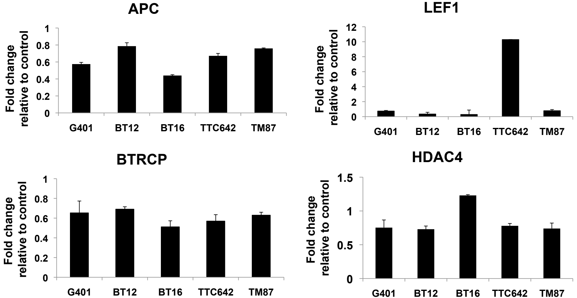
Supplemental Figure 4 : Expression of \beta -catenin/TCF targets in MRT cell lines. Expression of APC , BTRCP , LEF1 , and HDAC4 in G401, BT12, BT16, TTC642 , and TM87 cells after SNF5 re-introduction.
