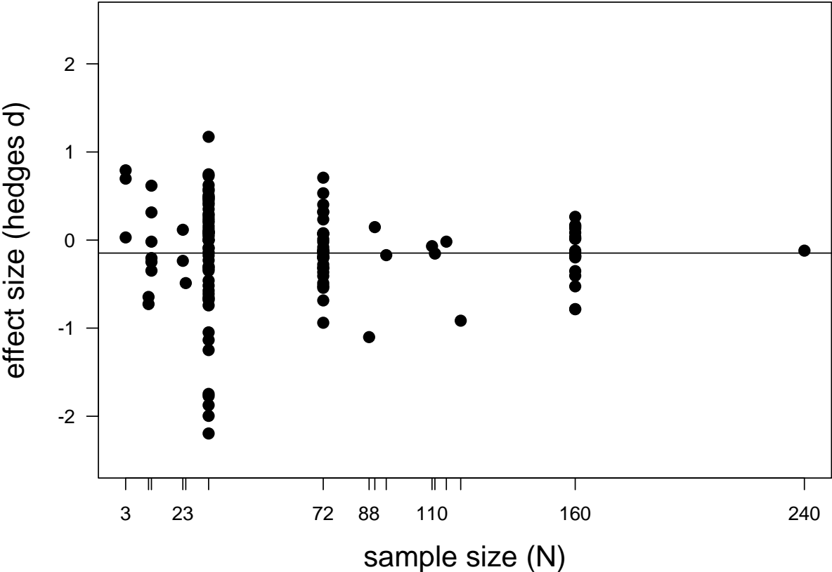
Figure 4. Funnel plot analysis of sample size against the Hedges' d value.
