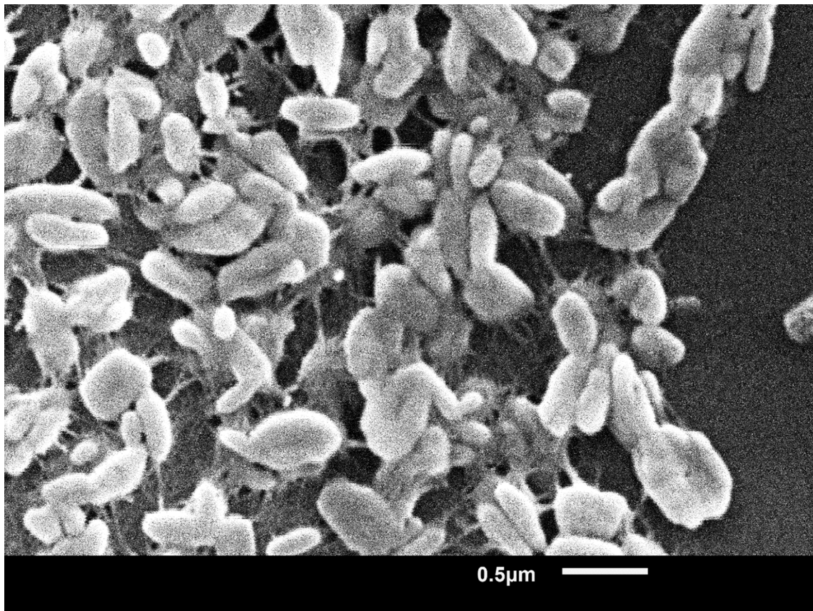
Figure S-6. SEM image of [Cp CoI 2 ]-SWCNT.
