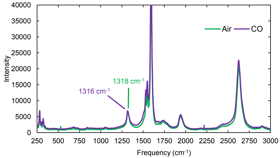
Figure S-5. Raman spectra of [Cp CoI 2 ]-SWCNT composite recorded under air and under 1 atm CO.
