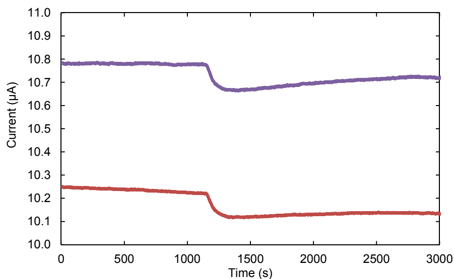
Figure S-2. Raw current traces of two [ \text{Cp}^{\wedge}\text{CoI}_2 ]-SWCNT devices exposed to 3000 ppm CO.
