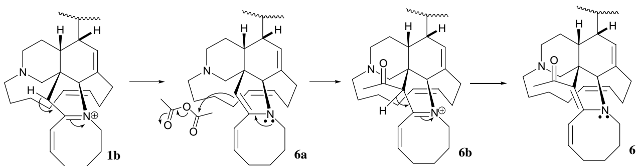
Scheme S1. Plausible mechanism of formation of compounds 6 and 9 .
