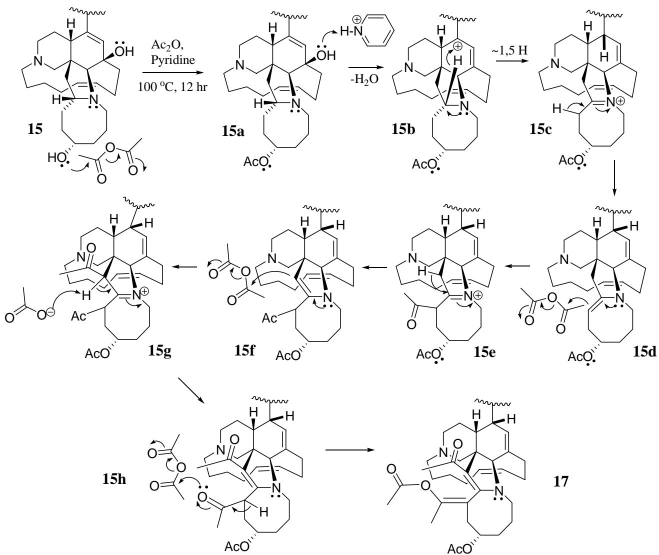
Scheme S2. Plausible mechanism of formation of compound 17 .
