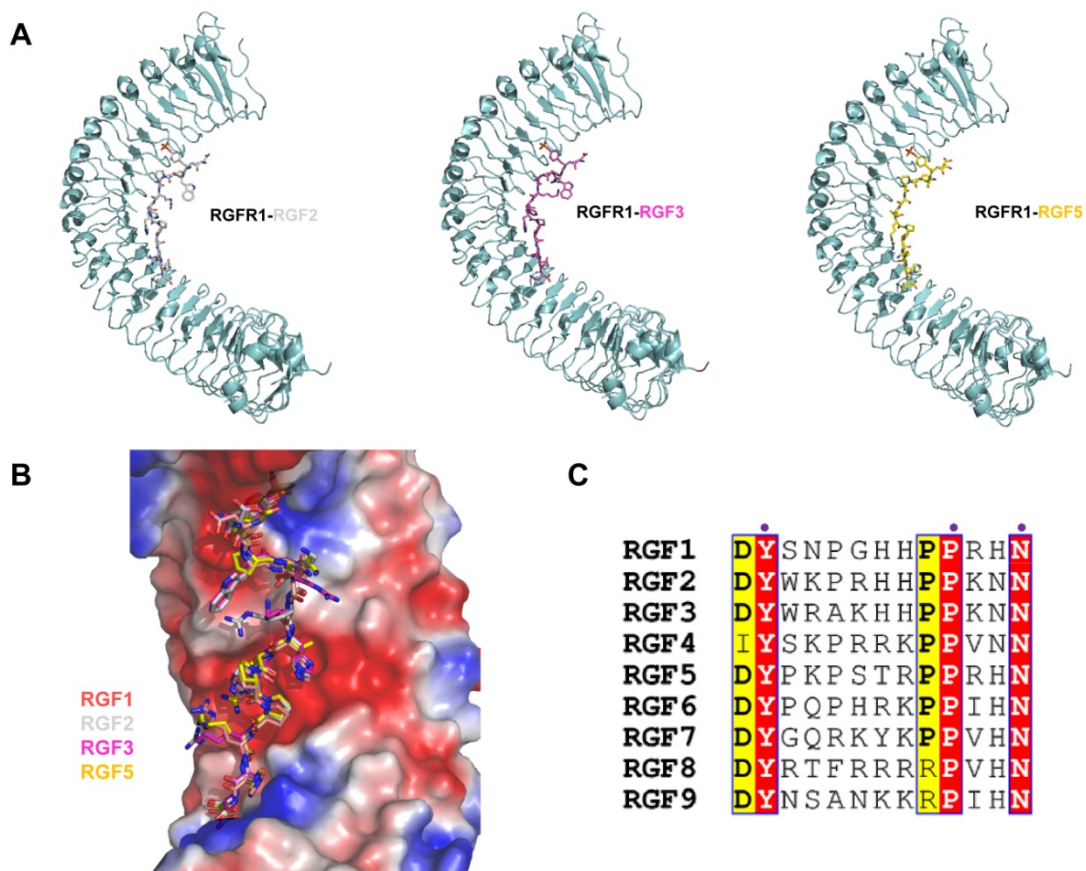
Figure S3 Conserved recognition mechanism of RGFs by RGFR1.
