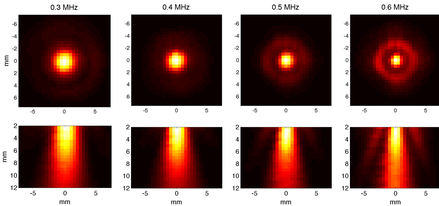
Figure S1: Normalized intensity plots measured by hydrophone for the Planar 500 kHz transducer setup (Experiment A) in the transverse plane (upper row, z = 2\text{mm} ) and the axial plane (bottom row)
