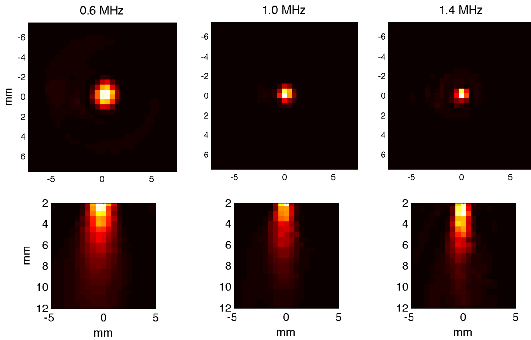
Figure S2: Normalized intensity plots measured by hydrophone for the Focused 1 MHz transducer setup (Experiment B) in the transverse plane (upper row, z = 2\text{mm} ) and the axial plane (bottom row)
