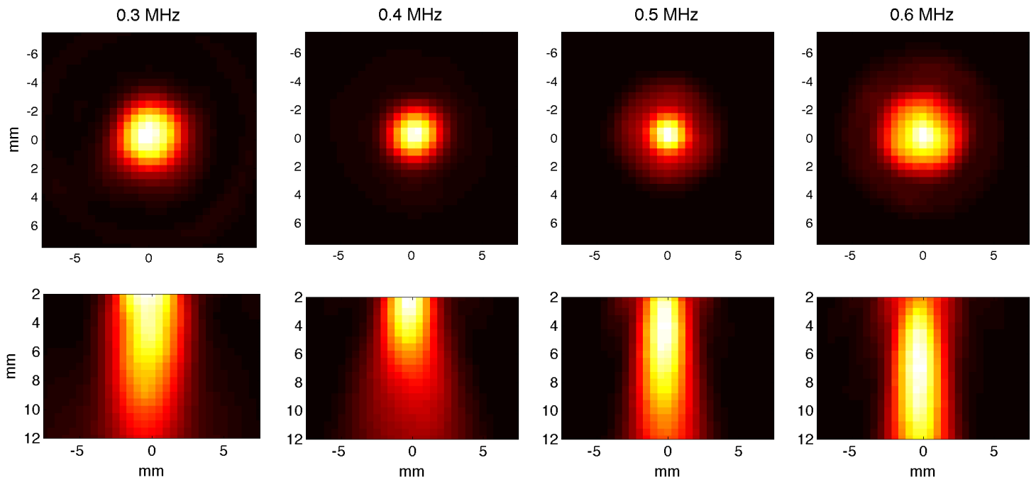
Figure S4: Normalized intensity plots measured by hydrophone for the Planar 500 kHz transducer setup (Experiment D) in the transverse plane (upper row, z = 2\text{mm} ) and the axial plane (bottom row)
