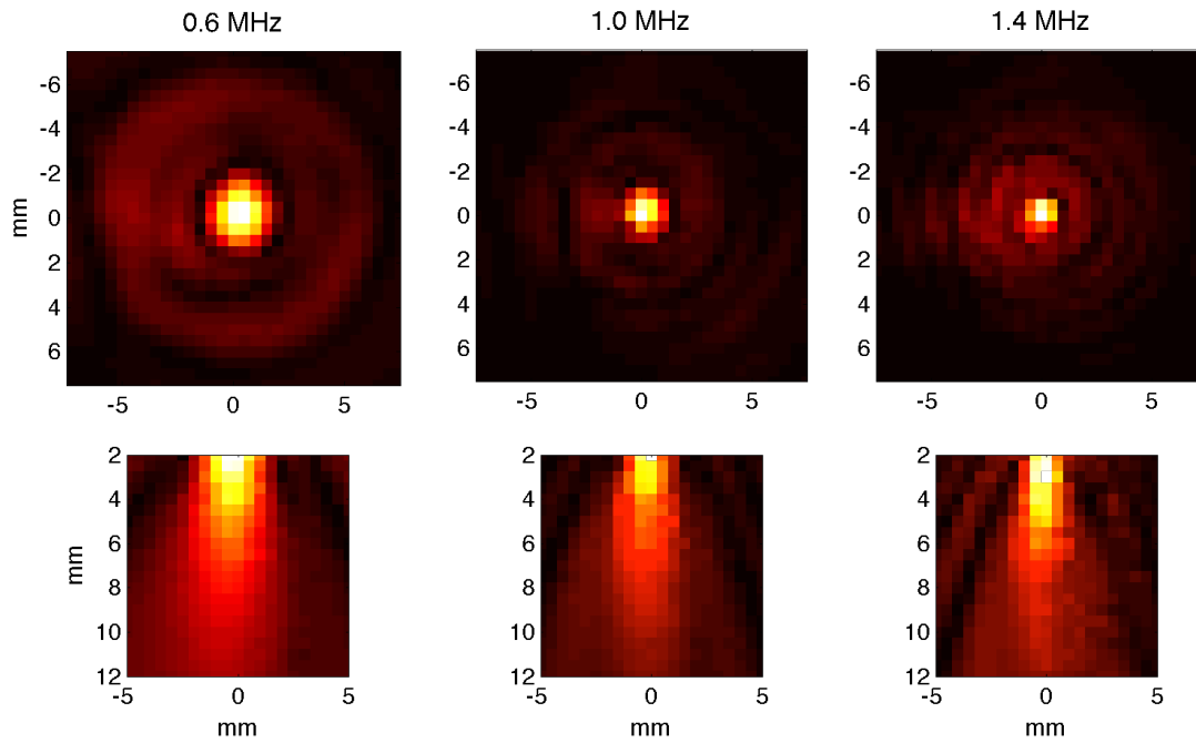
Figure S6: Normalized pressure plots measured by hydrophone for the Focused 1 MHz transducer setup (Experiment B) in the transverse plane (upper row, z = 2\text{mm} ) and the axial plane (bottom row).
