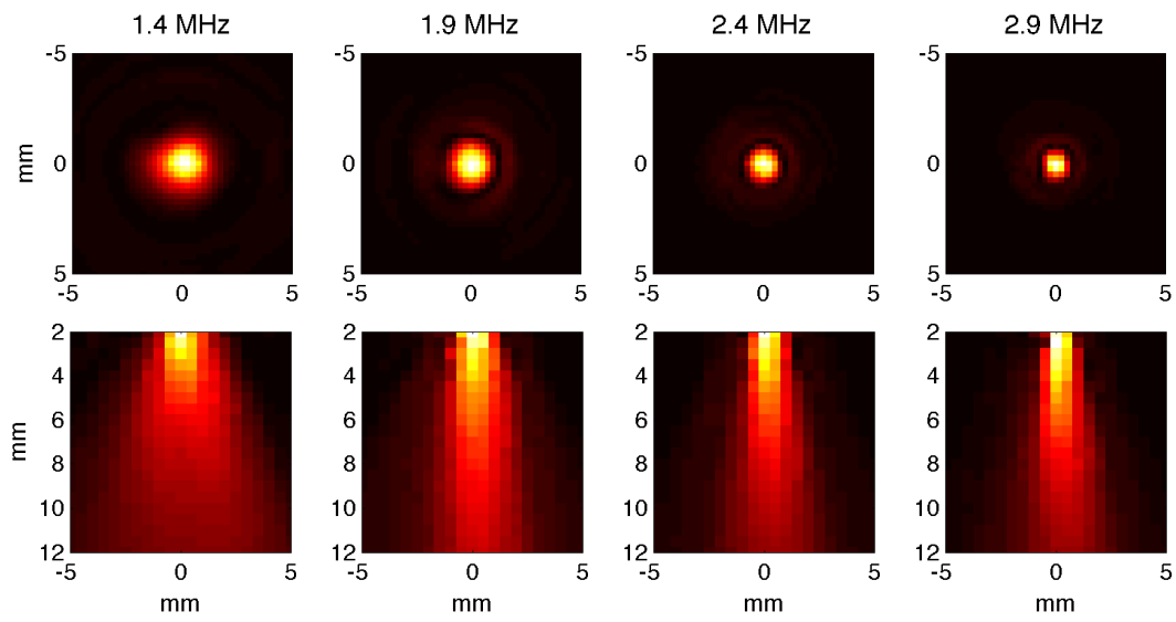
Figure S7: Normalized pressure plots measured by hydrophone for the Focused 2.25 MHz transducer setup (Experiment C and E) in the transverse plane (upper row, z = 2\text{mm} ) and the axial plane (bottom row).
