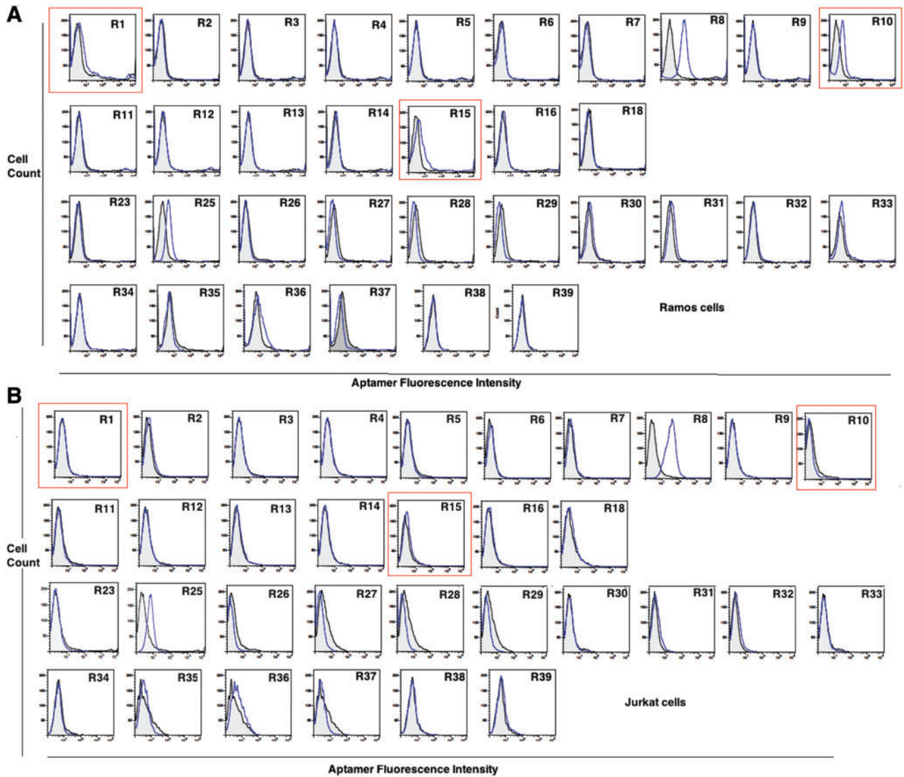
SUPPLEMENTARY FIG. S3. Analysis of binding specificity of aptamers selected using ligand-guided selection against Ramos cells ( A ) and Jurkat.E6 cells ( B ). FITC-labeled aptamers and random library were incubated with 1.0 or 0.5 \times 10^5 Ramos cells on ice for 45 min to 1 h. After washing twice with 0.5 or 1 mL of wash buffer, the sample was reconstituted in 250 \mu L of wash buffer and analyzed by flow cytometry by counting 5000 events. FITC, fluorescein isothiocyanate.
