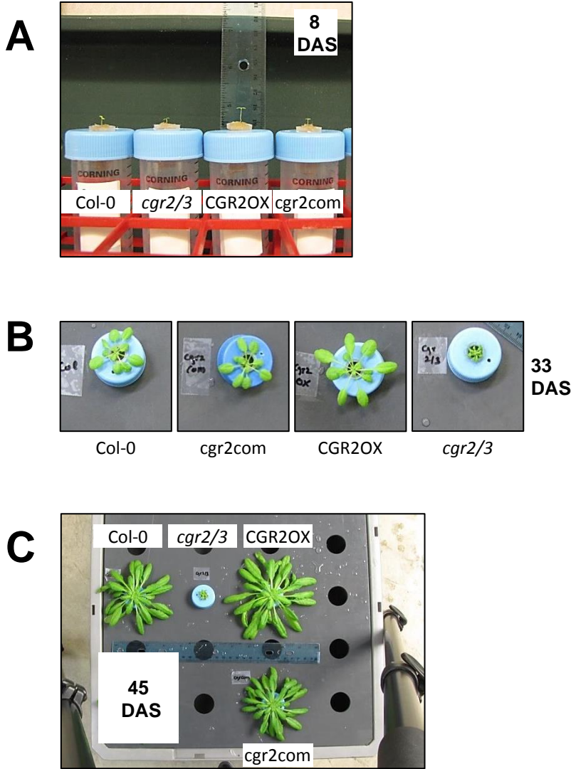
Supplemental Figure S2. Hypocotyl and rosette size in Arabidopsis with altered CGR2 and CGR3 expression. (A) Photographs comparing the height of the hypocotyls in 8-day old seedlings, and comparisons of rosette sizes in (B) 33-day and (C) 45-day old plants are presented for Col-0, cgr2com, CGR2OX, and cgr2/3.
