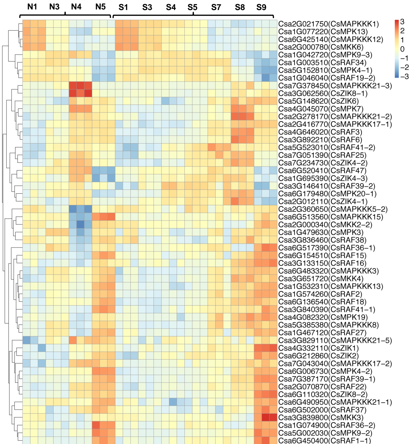
Supplemental Figure S3. Expression of MAP kinase family genes across developmental stages in the normal ovary and super ovary.
