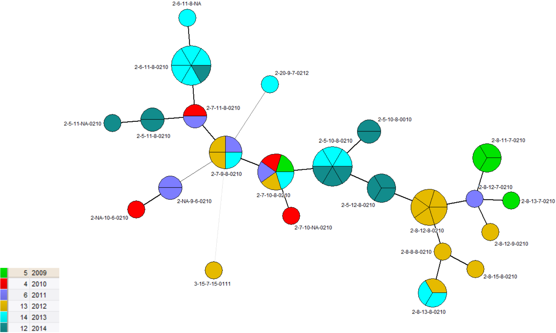
Figure S1. Minimum-spanning tree analysis of MLVA (multiple-locus variable-number tandem-repeats analysis) data of 54 Salmonella Typhimurium isolates from the Oriental Province, DRC, 2009-2014. Each circle displays a unique MLVA type, with different colours indicating the year of collection of isolates.
