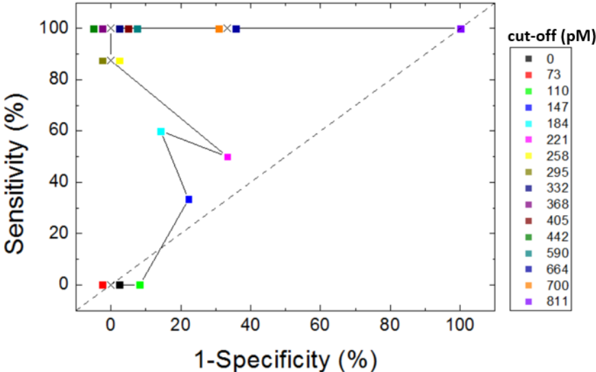
Figure S1: Receive Operating Characteristic (ROC) curve for the NutriPhone human trials. The legend shows the B12 cut-off points, and the dotted line shows the reference line.
