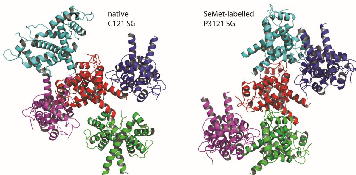
Figure S1 Different crystal packings in the two different crystal forms of Caprin-1 dimer. Five homodimeric Caprin-1 structures are shown in different colours.
