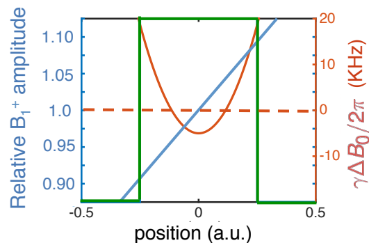
1D numerical phantom with \Delta B_0 field and linear B_1^+ amplitude field
