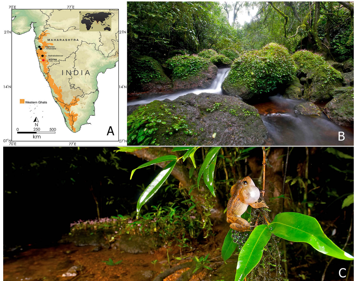
Figure S1 Study site and breeding habitat of Nyctibatrachus humayuni . (A) Distribution of N. humayuni in the Western Ghats of India. Study site is marked in red. (B) A mountain stream flowing over laterite rocks with overhanging vegetation, which is the typical breeding habitat of N. humayuni in the forest at Humbarli village, Koyna. (C) An adult male of N. humayuni is seen calling from overhanging vegetation.
