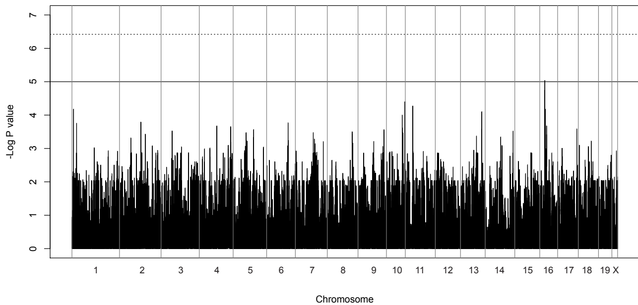
Figure S1. Genome-wide association mapping using EMMA.
