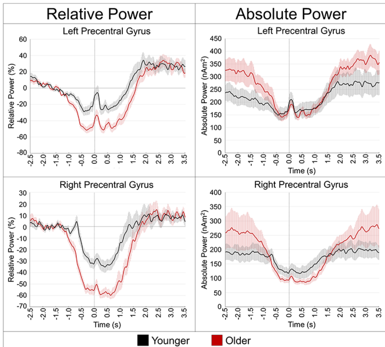
Figure S1. Absolute and relative temporal evolution of the alpha ERD response. Voxel time series were extracted from the peak voxels of the left precentral gyrus (top panel) and right precentral gyrus (bottom panel) to more precisely examine the dynamics of the alpha ERD in younger (black line) and older adults (red line). Time (in s, movement onset = 0.0 s) is denoted on the x-axis, while power is shown on the y-axis. The left panel shows each response as percentage relative to baseline (-1.8 to -1.2 s), while the right panel shows the absolute power (in \text{nAm}^2 ). The shaded area around each line denotes the standard error of the mean (SEM).
