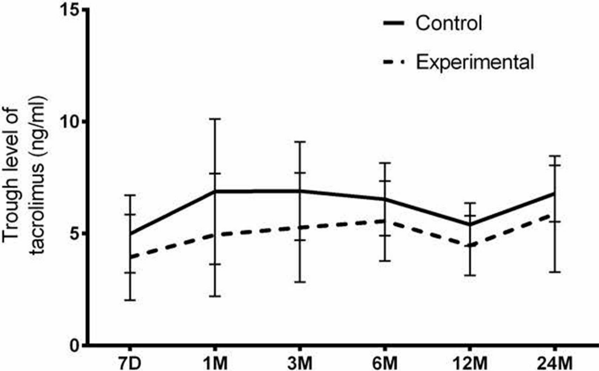
Supplementary Figure S1: Trough level of tacrolimus over time in 32 patients.
