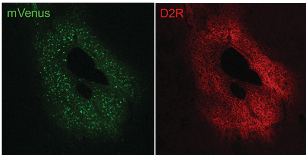
Figure S1. Representative images demonstrating that mVenus and D2R are stably and robustly overexpressed in the NAc 6 months after viral transduction. Note the lower endogenous D2R immunofluorescence in surrounding striatal regions.
