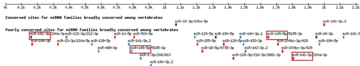
S2 Fig. Predicted binding sites on target transcripts.
