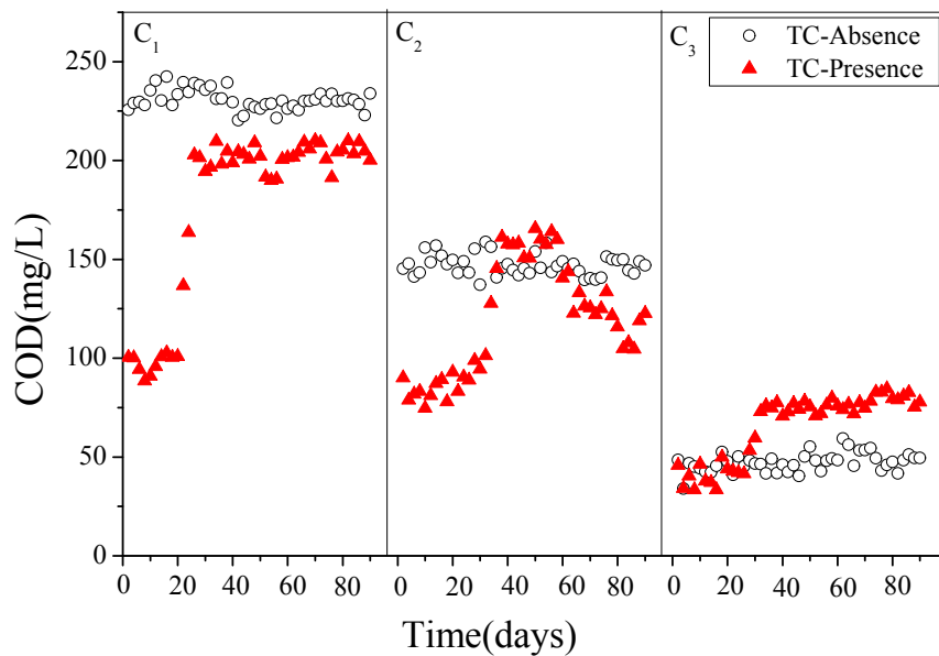
Figure S1 | Responses of effluent COD in each compartment of the reactor.
