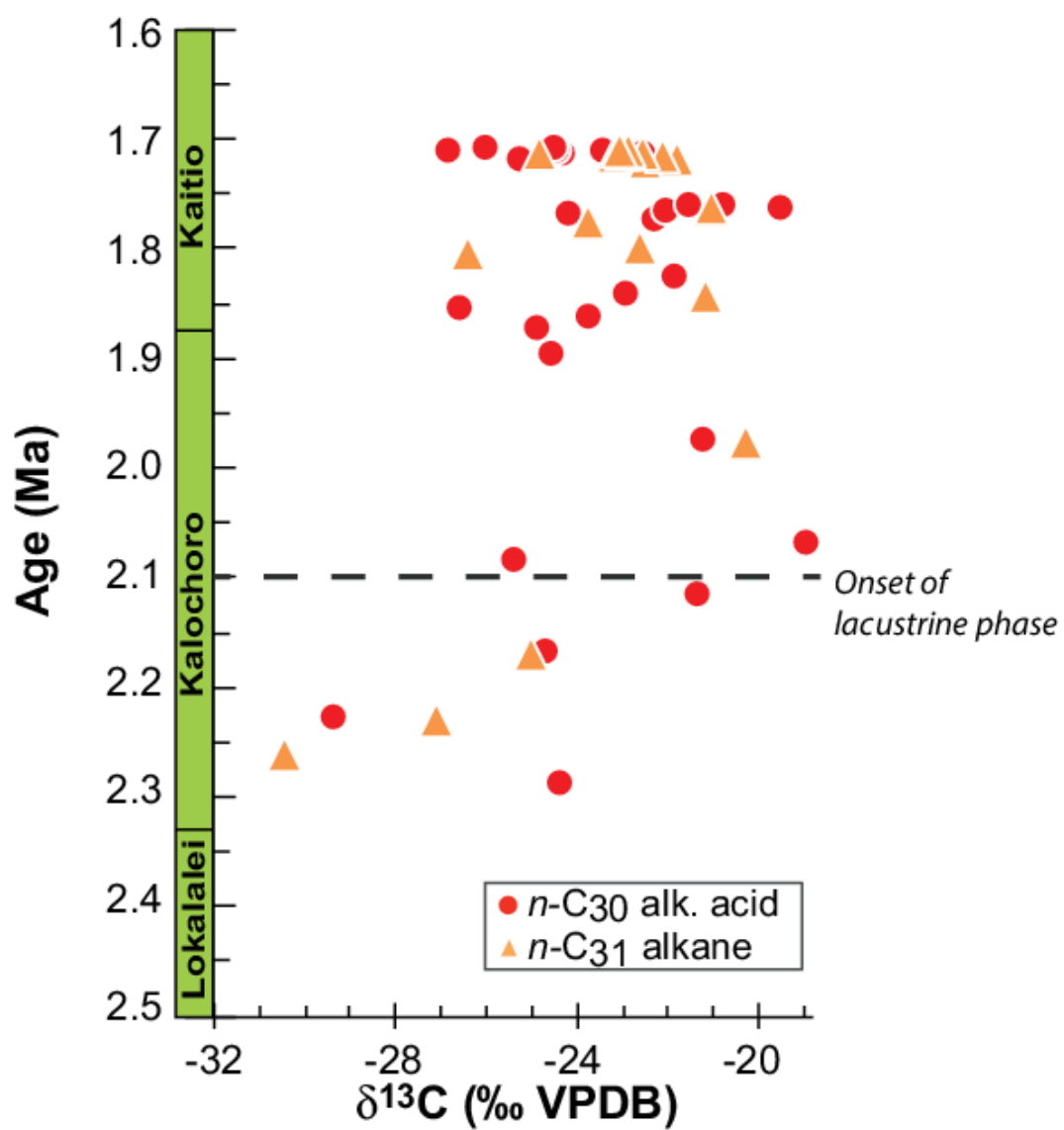
Figure S1. The \delta^{13}\text{C} values of n\text{-C}_{30} alkananoic acids and n\text{-C}_{31} alkanes versus age for Nachukui Formation samples.
