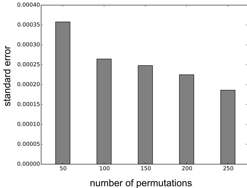
Standard error of CDF estimation (40 samples)
