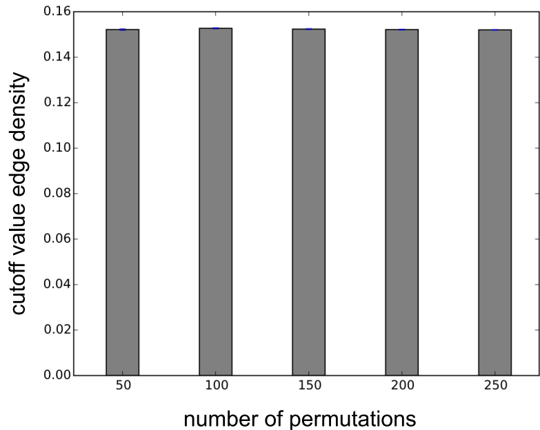
CDF estimation in dependency of the number of permutations
