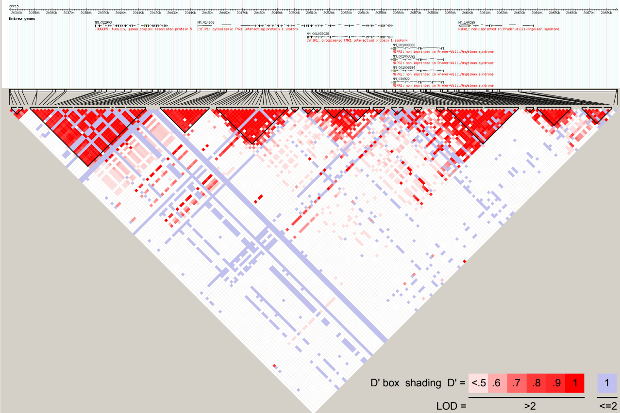
S1 Figure. Linkage disequilibrium (LD) structure of the Breakpoint 1 to Breakpoint 2 locus.
