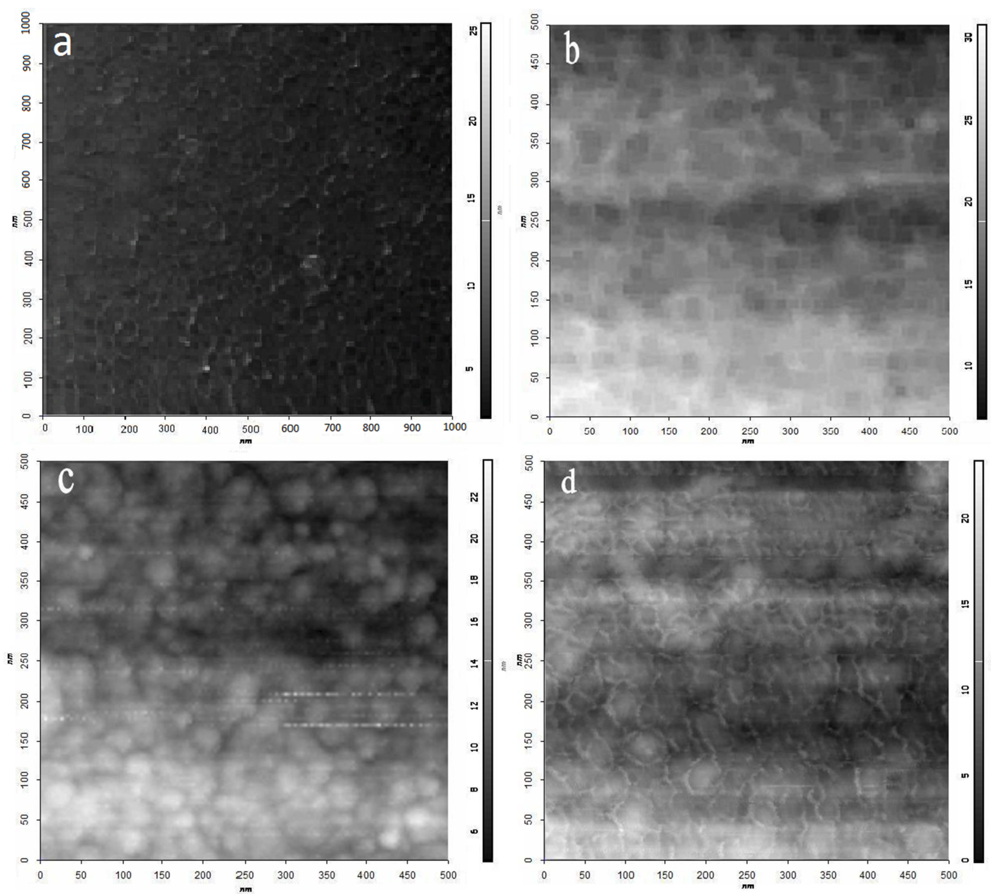
Fig.1. AFM pictures of bare gold (a), cysteamine (b), antibody (c), laminin-5 (d) on the chip.
