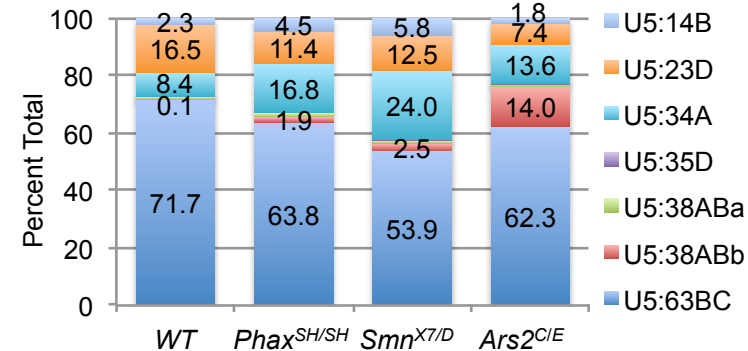
Supplemental Figure S3. Relative abundance of snRNA isoforms in snRNP biogenesis mutants: (A) U1 snRNA paralogs; (B) U2 snRNA paralogs; (C) U4 snRNA paralogs; and (D) U5 snRNA paralogs. Identical isoforms are listed together.
