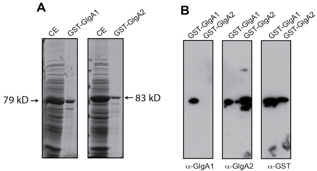
Supplemental Figure 7. ^{14}\text{C} -Recombinant proteins GlgA1 and GlgA2. The recombinant proteins GST-GlgA1 and GST-GlgA2 were extracted and observed by sodium dodecyl sulfate polyacrylamide gel electrophoresis (9% SDS-PAGE). (B) Western blot analysis of purified recombinant protein GST-GlgA1 and GST-GlgA2 of Cyanobacterium sp CLg1 using the antibodies \alpha -GlgA1 and \alpha -GlgA2 of Synechocystis PCC6803 and polyclonal antibodies raised against glutathione S-transferase ( \alpha -GST).
