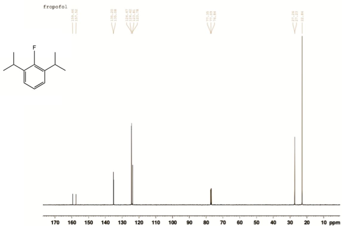
Supplementary Figure 2. 13 C NMR spectra for 2-fluoro-1,3-diisopropylbenzene, or “fropofol”
