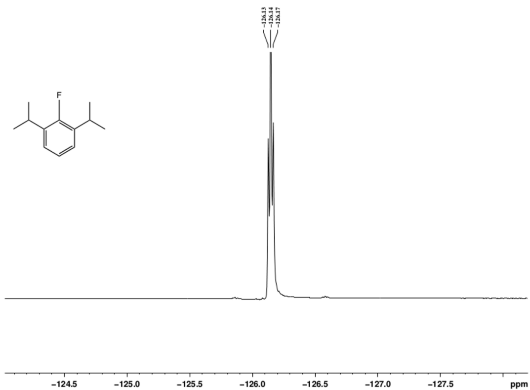
Supplimentry Figure 3. 19 F NMR spectra for 2-fluoro-1,3-diisopropylbenzene, or “ fropofol ”
