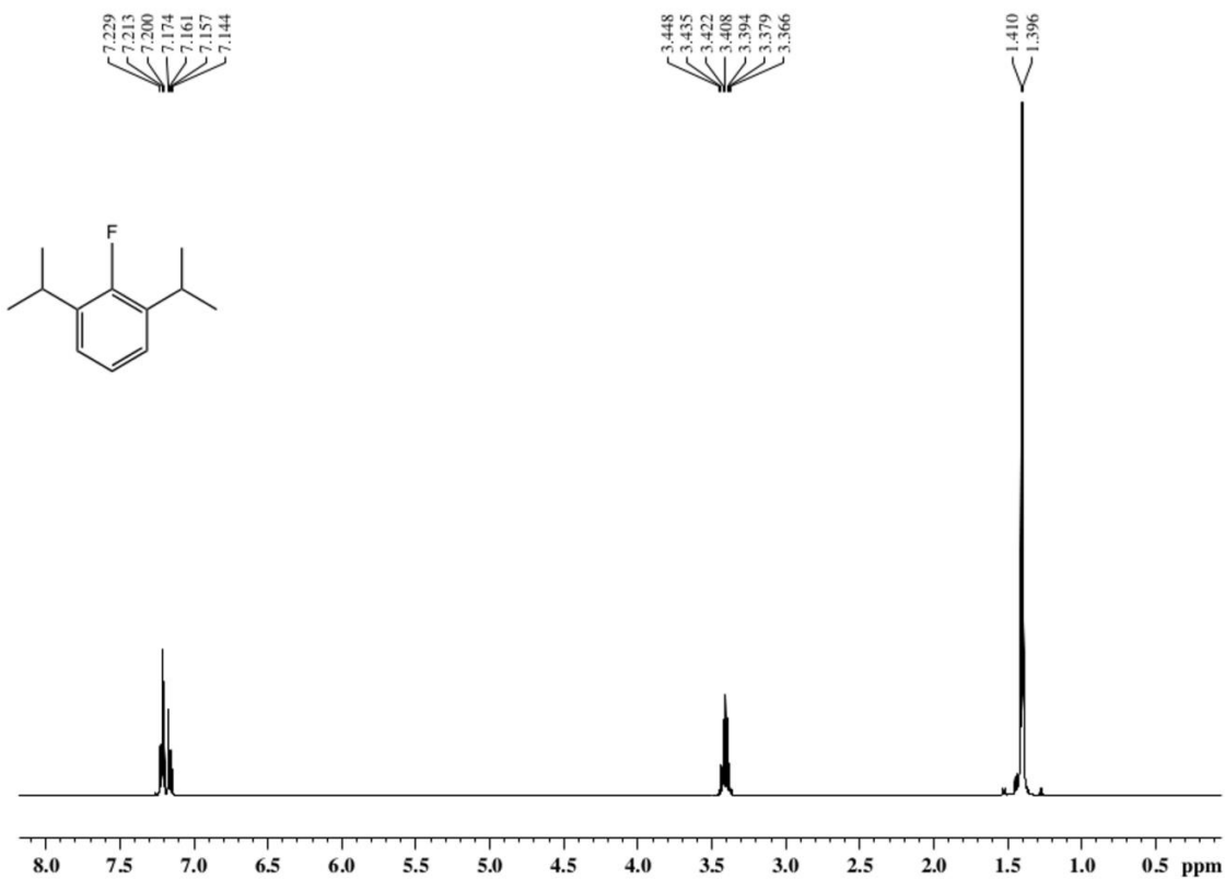
Supplementary Figure 1. 1 H NMR spectra for 2-fluoro-1,3-diisopropylbenzene, or “ fropofol ”
