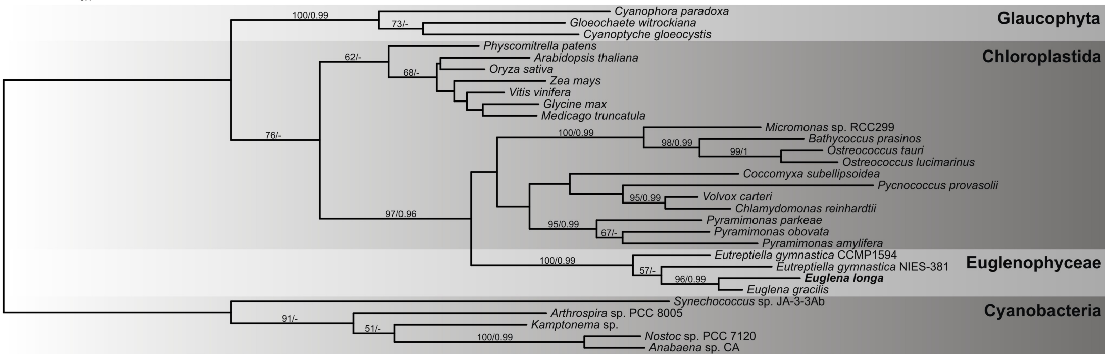
Figure S3. Phylogenetic tree of RCA protein sequences. The maximum-likelihood tree was inferred with RAxML using the LG+ \Gamma substitution model. The bootstrap support values and posterior probabilities (from PhyloBayes) are indicated at branches when higher than 50% and 0.95, respectively. E. longa is in bold.
