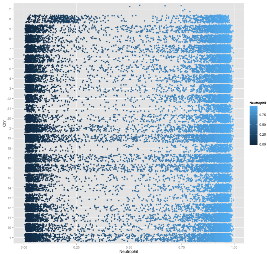
Figure S3. Chromosome-wise methylation of human neutrophils. The y-axis shows chromosomes and x-axis shows methylation of each of the comparison fragments (scale of 0 to 1.0). Note: the data shown here are the same as in Figure 1a, but in Fig S3 they are separated by chromosome.
