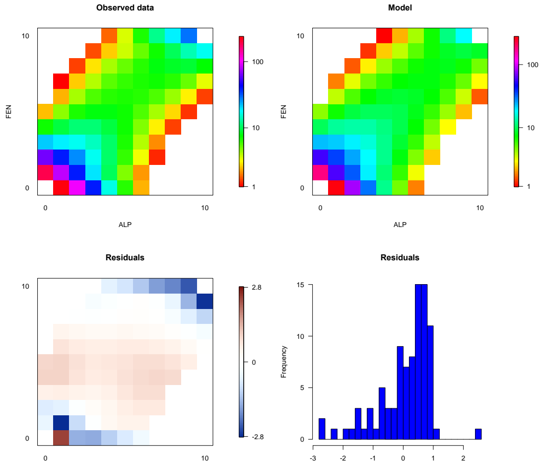
Figure S3. Comparison of two-dimensional site frequency spectra inferred by fastsimcoal2 with that of observed data. Allele frequencies are projected into a 10×10 grid. Multinomial comparison was applied by computing Anscombe residuals.
