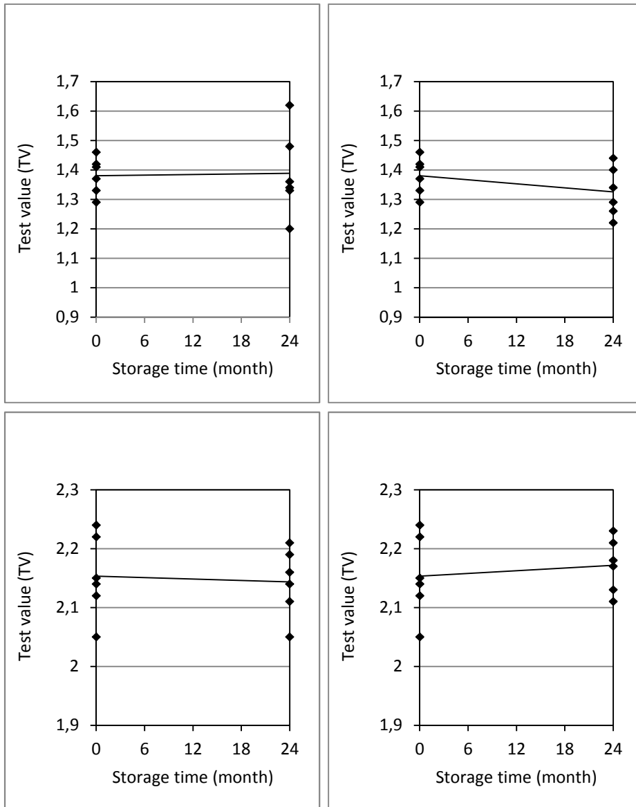
Fig. S2. Results of the 2-year stability study of IRMM-359b and IRMM-359c using the ESM/VIDAS for analysis. The obtained results per individual time point and the respective regression line are shown. Upper part: IRMM-359b, storage temperature 4 0 C (left) and -20 0 C (right). Lower part: IRMM-359c, storage temperature 4 0 C (left) and -20 0 C (right)
