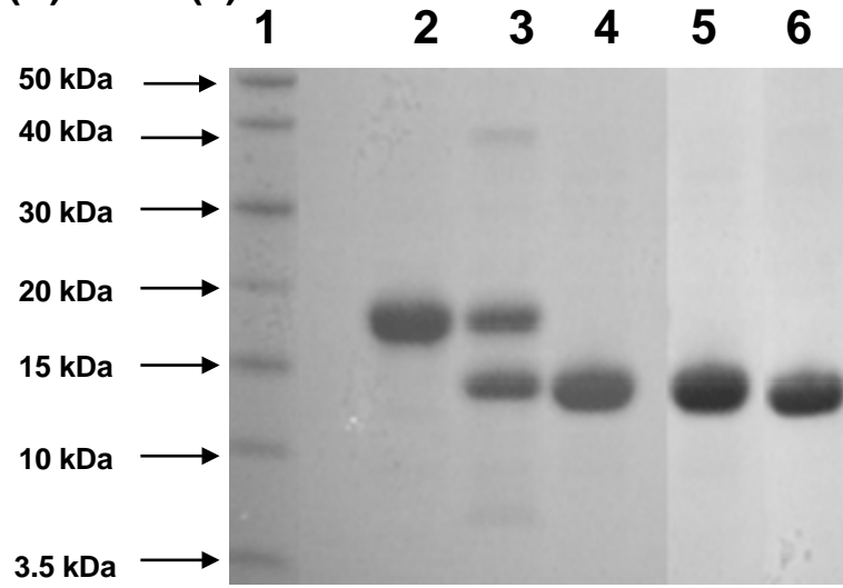
(A) BRD2(2)
