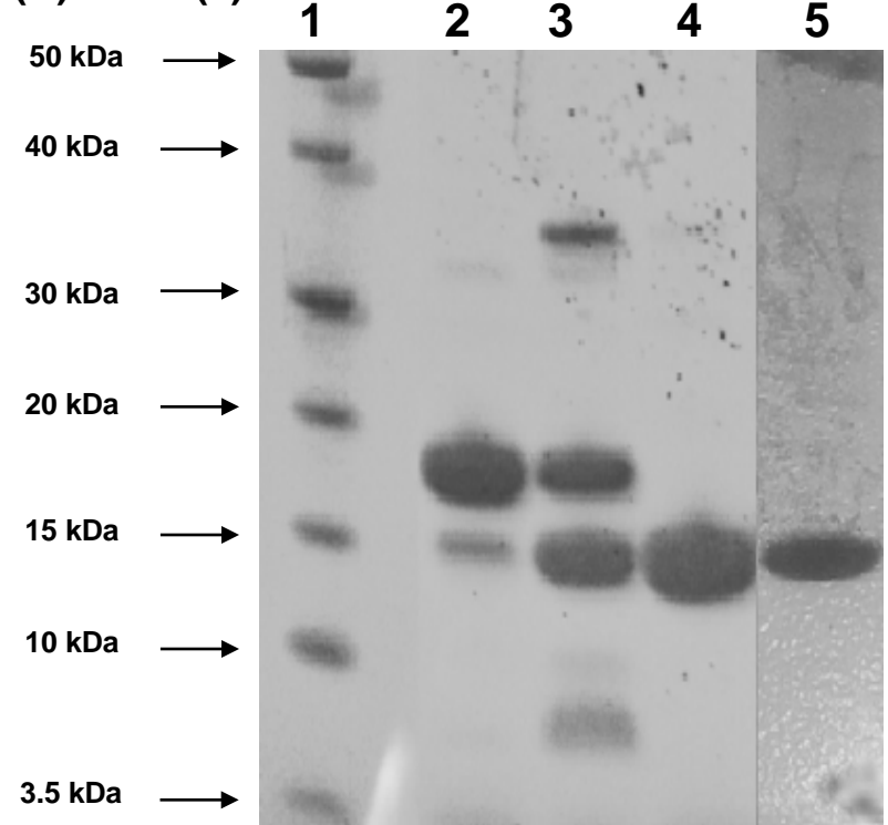
(C) BRD4(2)
