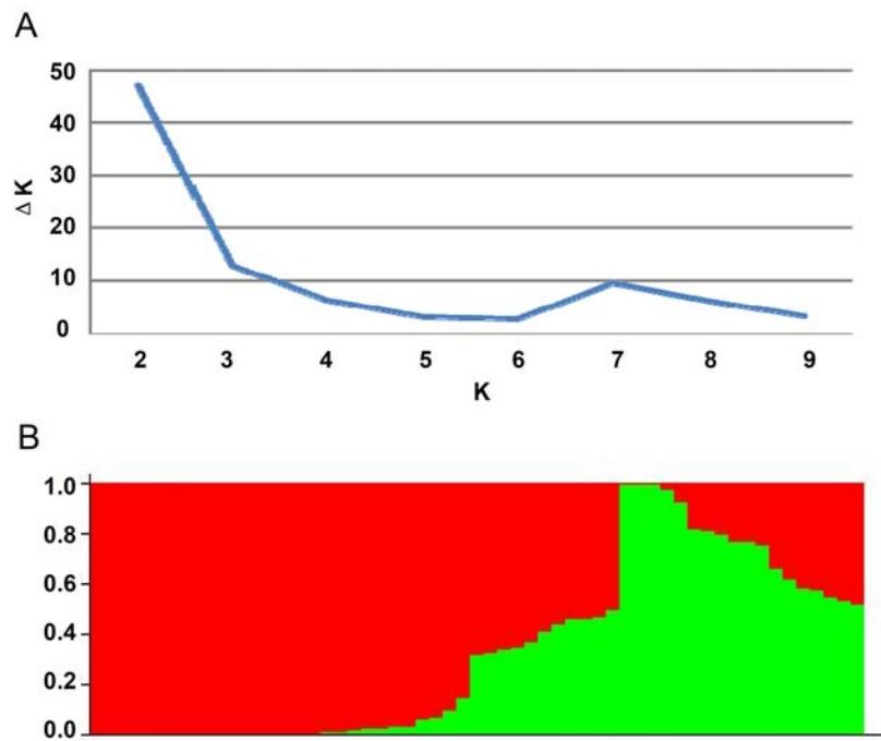
Figure S1 Population structure of 56 soybean accessions
