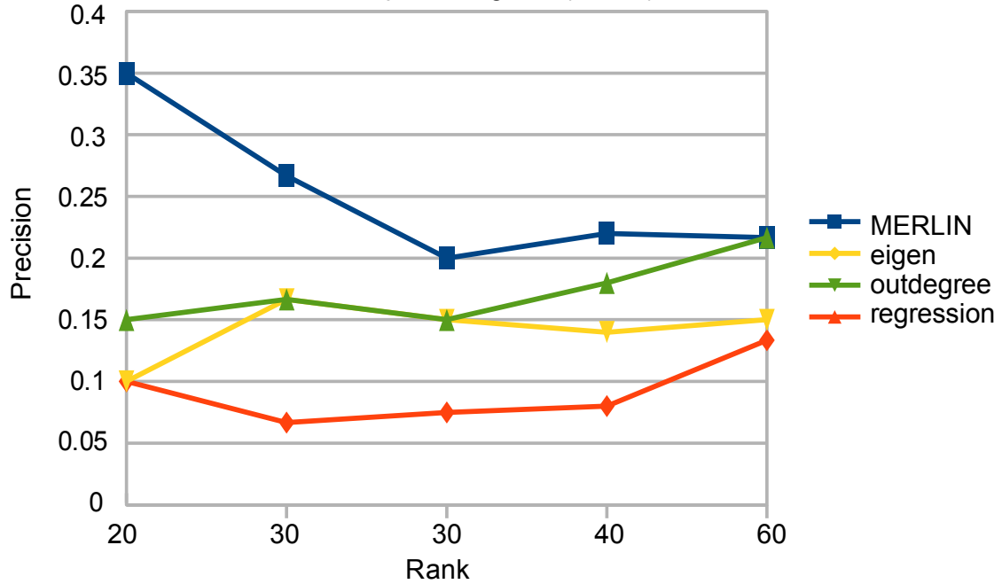
Precision of top ranked genes (Mouse)
