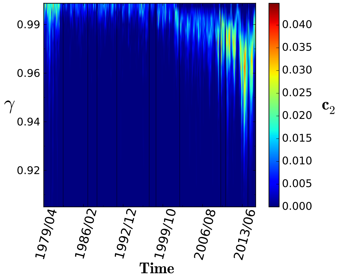
Figure S1: Heatmap with an exploration of the fraction of nodes in clusters of size 2, c_2 , as a function of time and of \gamma for functional networks extracted daily over 30 years of data on the mean Sea Surface Temperature T monitored in the NINO3.4. The spatial resolution is 0.5 arc degrees.
