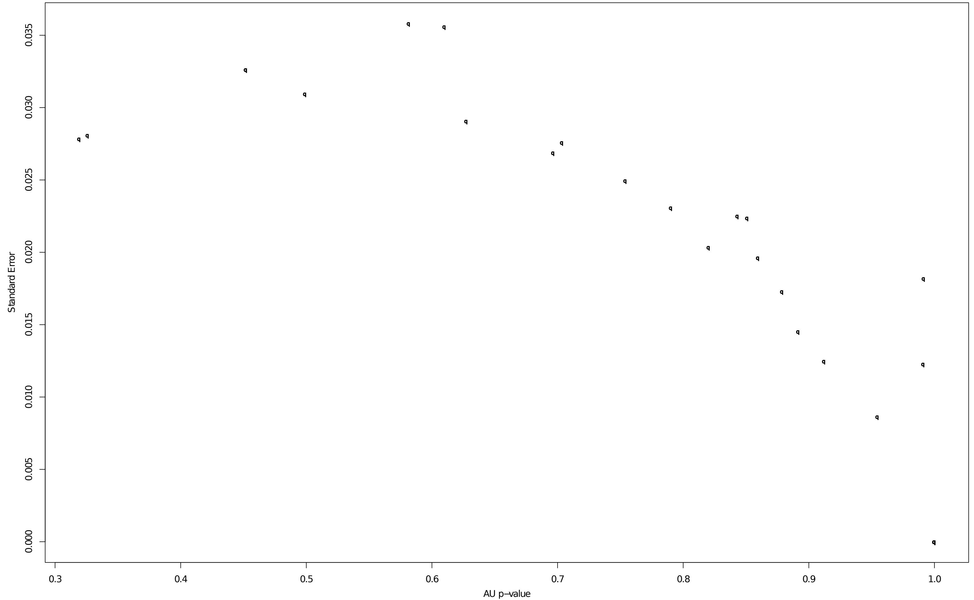
S1 Fig: Standard error of each p-value of multi-scale bootstrap in Fig 1
