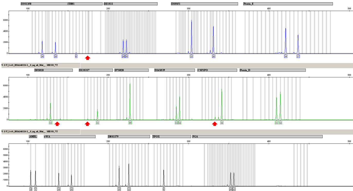
Supplementary Figure S5. An electropherogram of Powerplex PCR reaction. Top lines show STR profile in 7T tumor genomic DNA; no peak imbalance, indicative of a mixture in the sample, was noted. Bottom profile shows STR profile of the primary cell line MESO-7T. Arrows indicate positions of allele alterations compared to the parental genomic DNA.
