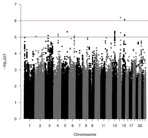
Supplementary Fig. 2. Manhattan plots. (A) Manhattan plot of bone mineral density (BMD) at the lumbar spine. (B) Manhattan plot of BMD at femur total.
