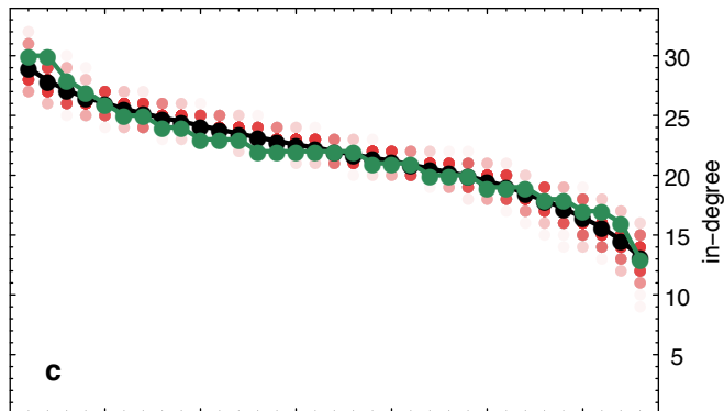
mouse
