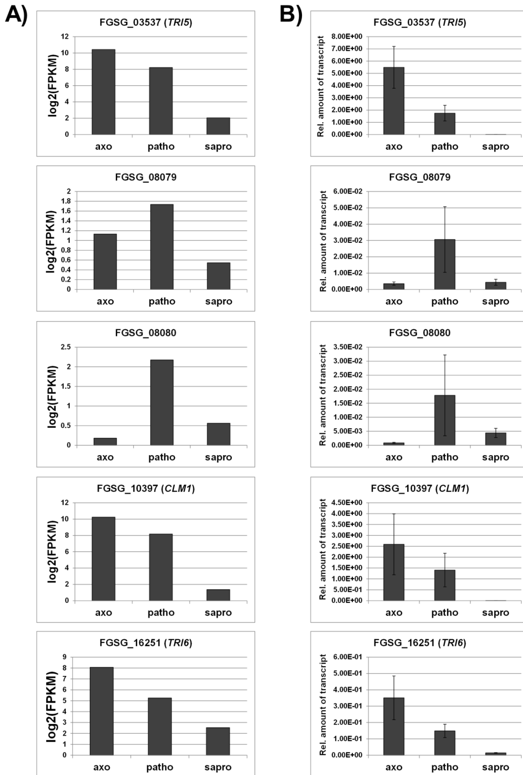
Figure S1: Verification of relative transcript abundances found in RNA-seq analysis (A) by RT-qPCR (B). Details of RNA-seq analysis and primers as well as conditions for RT-qPCR are described in Materials and Methods (Patho... pathogenic growth; sapro... saprophytic growth; axo... axenic growth on L-ornithine).
